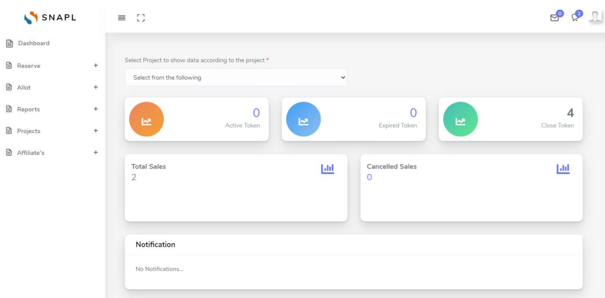
Figure 3 SPO dashboard
