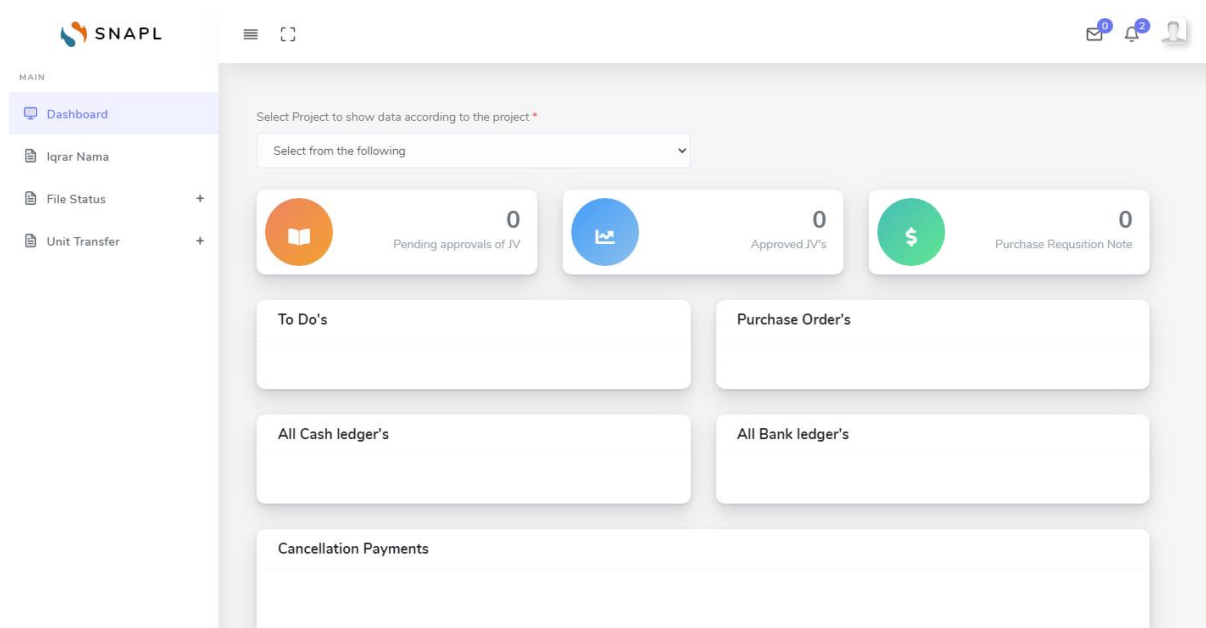
Figure 6 IRO dashboard
