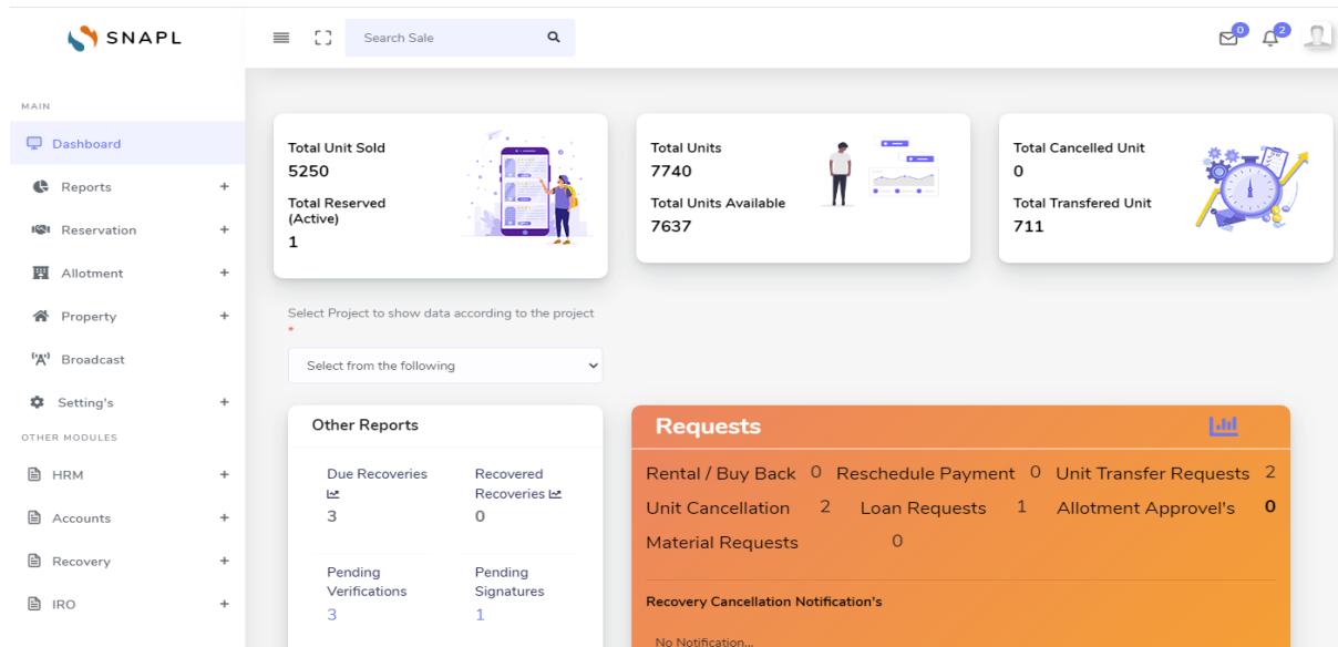
Figure 1 Admin dashboard
