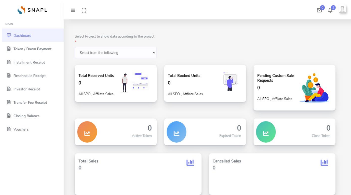
Figure 4 Cashier dashboard
